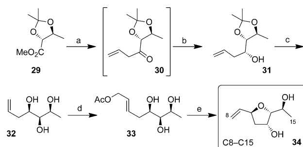
Scheme 5. Synthesis of the C8–C15 fragment of (–)-obtusallene III ( 2 ). Reaction conditions: a) \text{MeNH}(\text{OMe}) \cdot \text{HCl} , LiHMDS, THF, –20 °C \rightarrow 0 °C, then \text{H}_2\text{C}=\text{CHCH}_2\text{MgCl} ; b) K-Selectride, THF, \text{Et}_2\text{O} , –78 °C, 61% (over 3 steps); c) 2 M HCl, \text{H}_2\text{O} , vacuum, 85%; d) allyl acetate, second generation Grubbs' catalyst, \text{CH}_2\text{Cl}_2 , 82%; e) cond. A in Scheme 2, 35 °C, 78%, d.r. = 90:10.
