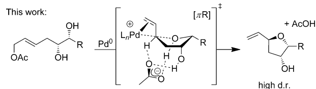
Scheme 1. Rationalized examples of CDC in the Tsuji–Trost reaction.
