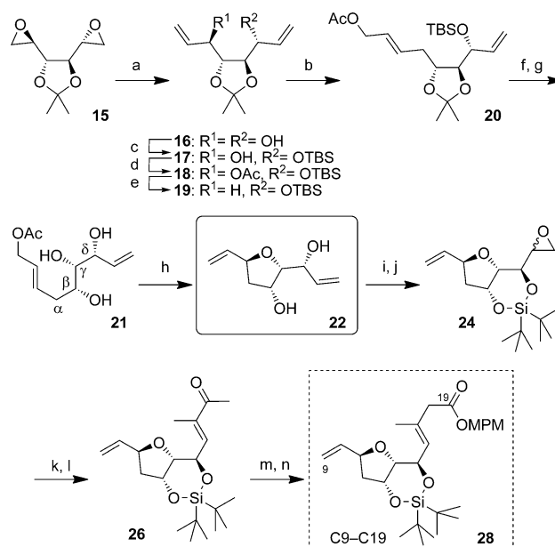
Scheme 4. Second generation synthesis of the C9–C19 fragment of (+)-oocydin A ( 1 ). Reaction conditions: a) n\text{BuLi} , \text{Me}_3\text{SiI} , THF, 45 °C, 76%; b) second generation Grubbs' catalyst, ( Z )-but-2-ene-1,4-diyl diacetate (neat), 45 °C, 74%; c) NaH, TBSCl, DME, 0 °C; d) \text{Ac}_2\text{O} , 4-DMAP, pyridine, RT, 98% (over 2 steps); e) [\text{Pd}_2(\text{dba})_3] , n\text{Bu}_3\text{P} , \text{HCO}_2\text{H} , \text{Et}_3\text{N} , THF, 60 °C, 97%; f) TBAF, THF, RT, 98%; g) \text{CeCl}_3 \cdot (\text{H}_2\text{O})_7 , oxalic acid, MeCN, reflux, 90%; h) cond. C in Scheme 2, 40 °C, 80% (d.r. = 90:10); i) VO(acac) 2 , t\text{BuO}_2\text{H} , PhMe, 90 °C, 75%; j) (t\text{Bu})_2\text{Si}(\text{OTf})_2 , 2,6-lutidine, TTBP, \text{CH}_2\text{Cl}_2 , 0 °C, 80%; k) rac -Co III -salen, \text{H}_2\text{O} , THF, RT, 80%; l) NaIO 4 , silica gel, \text{CH}_2\text{Cl}_2 , RT, then PO(OEt) 2 CHMeCOMe, NaH, THF, 0 °C, 83%; m) \text{CF}_3\text{COOCH}_2\text{CF}_3 , n\text{BuLi} , HMDS, THF, –78 °C, then \text{Et}_3\text{N} , \text{H}_2\text{O} , \text{MsN}_3 , MeCN, 35 °C, 50% (over 2 steps); n) \text{PhCO}_2\text{Ag} , \text{Et}_3\text{N} , MPMOH, THF, RT, 60%. acac = acetylacetonate, DMAP = dimethylaminopyridine, DME = 1,2-dimethoxyethane, HMDS = hexamethyldisilazane, TBAF = tetrabutylammonium fluoride, TBS = tert -butyldimethylsilyl, TTBP = 2,4,6-tri- tert -butylpyrimidine.
